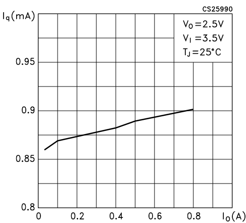
Figure 8. Quiescent current vs output current
