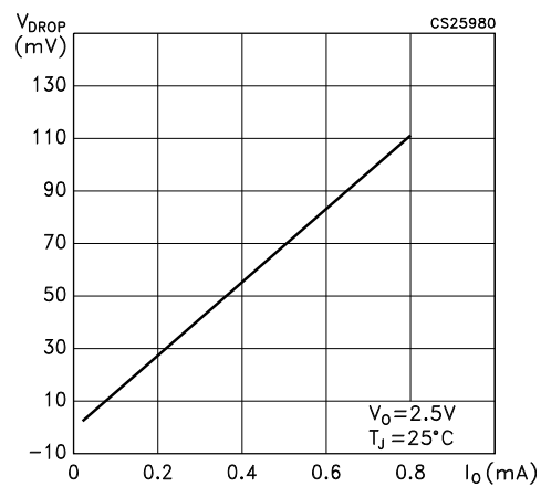
Figure 7. Dropout voltage vs output current
